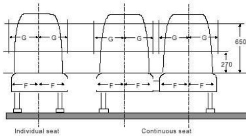
Figure 9A WIDTH OF PASSENGER SEATS
