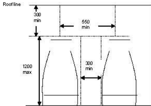
Figure 5 ACCESS TO EMERGENCY DOORS
