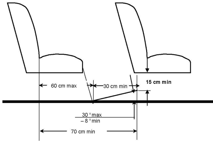
Figure 12 SEAT SPACING
