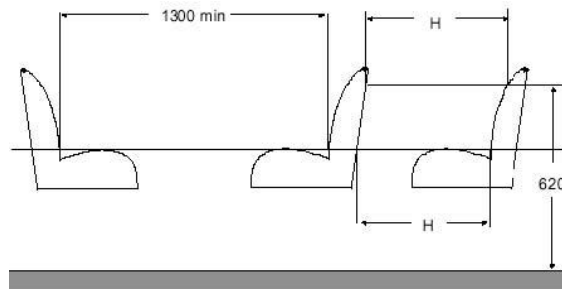
Figure 12 SEAT SPACING
