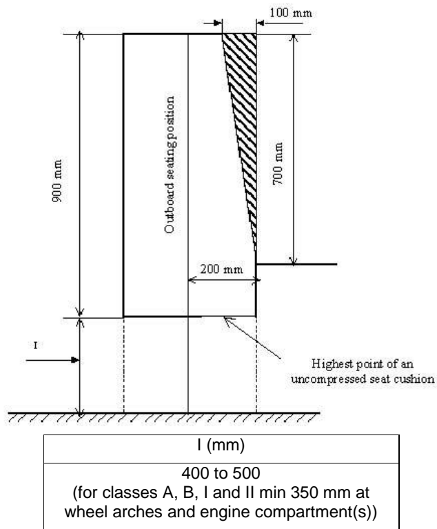
Figure 16 PERMITTED INTRUSION IN LOWER PART OF PASSENGER SPACE
