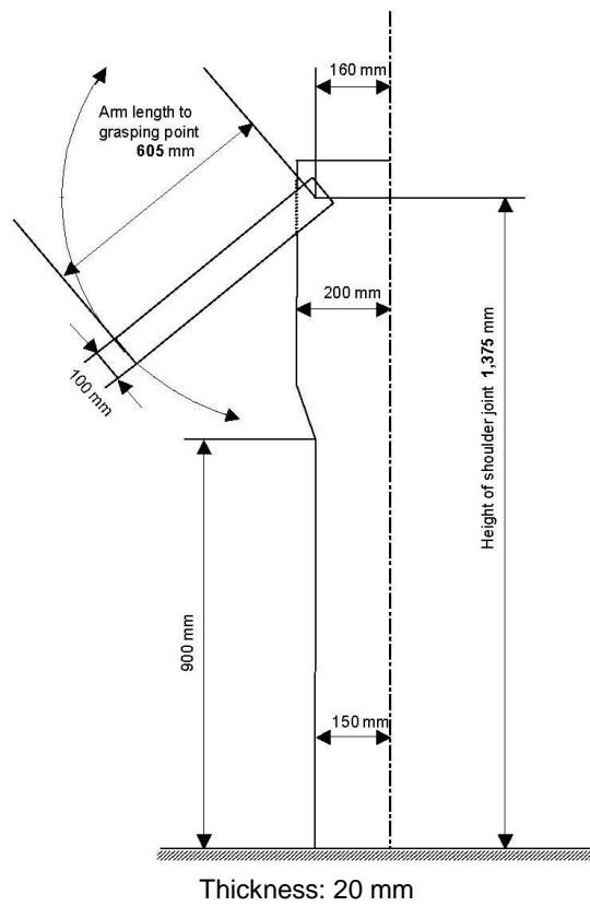
Figure 21 REFERENCE WHEELCHAIR
