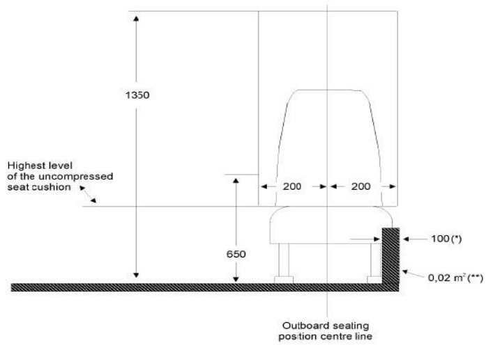
Figure 16 PERMITTED INTRUSION IN LOWER PART OF PASSENGER SPACE
