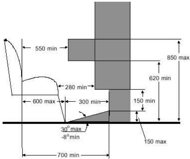
Figure 14 PERMITTED INTRUSION INTO SPACE ABOVE SEAT
