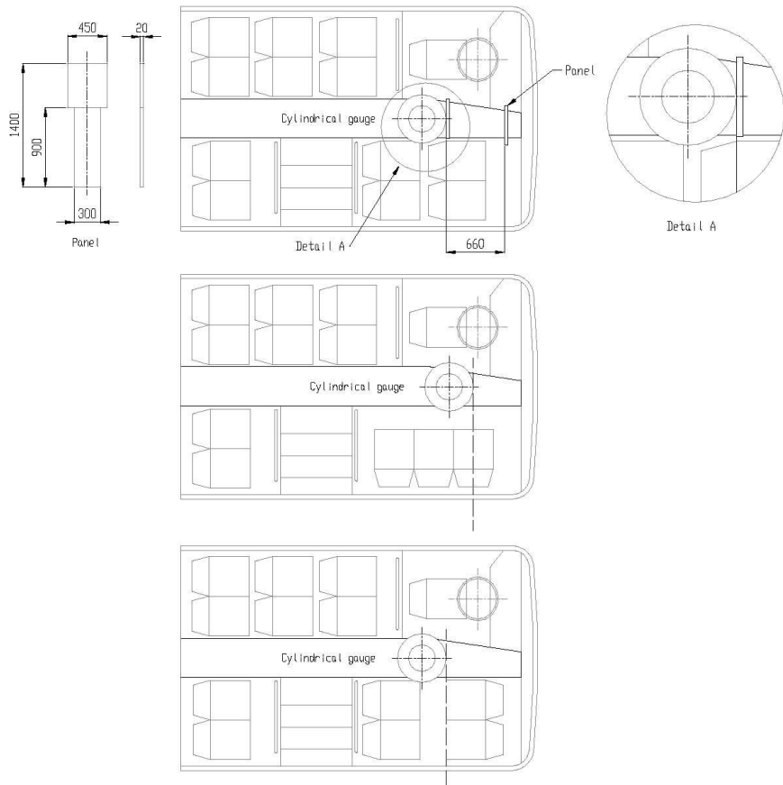
Figure 8 STEPS FOR PASSENGERS (see Annex 3, paragraph 7.7.7.)
