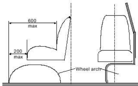
Figure 20 TESTING DEVICE FOR SITING OF HANDHOLDS
