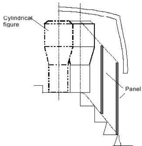
Figure 3 DETERMINATION OF UNOBSTRUCTED ACCESS TO DOOR
