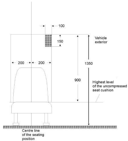
Figure 15 PERMITTED INTRUSION ABOVE A SEATING POSITION
