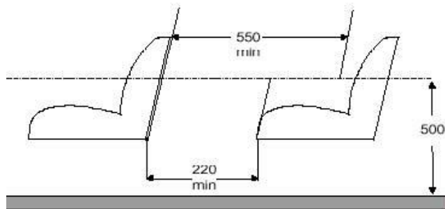
Figure 4 DETERMINATION OF UNOBSTRUCTED ACCESS TO DOOR
