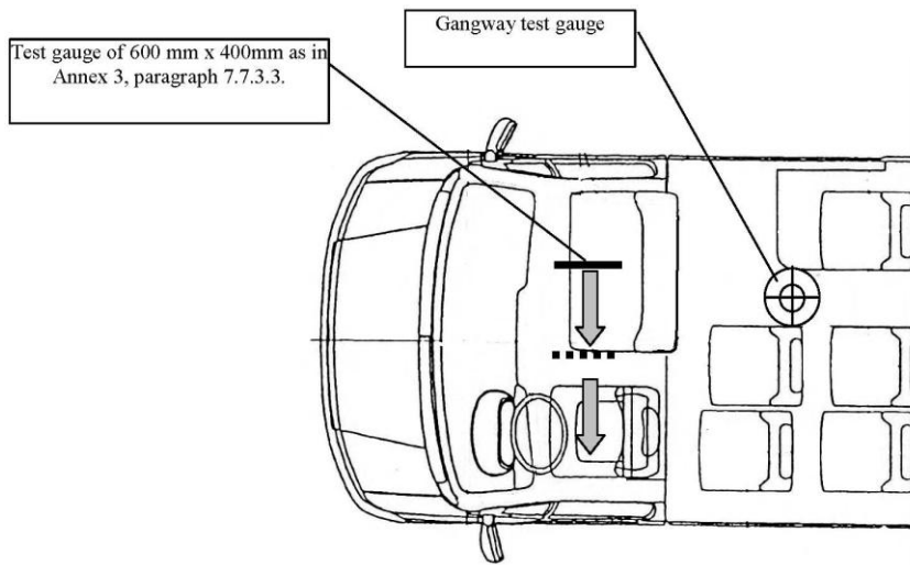
Figure 28 ACCESS TO DRIVER'S DOOR
